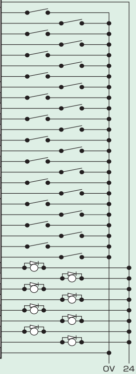
Wiring diagram
