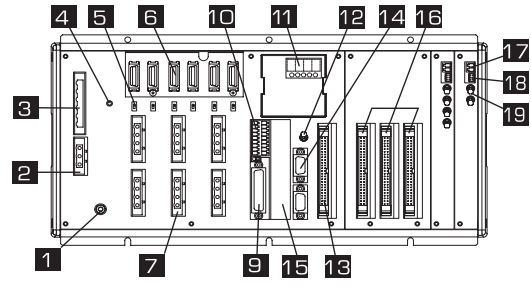
PQ type (with absolute brake unit + expansion base, 6-axis)
